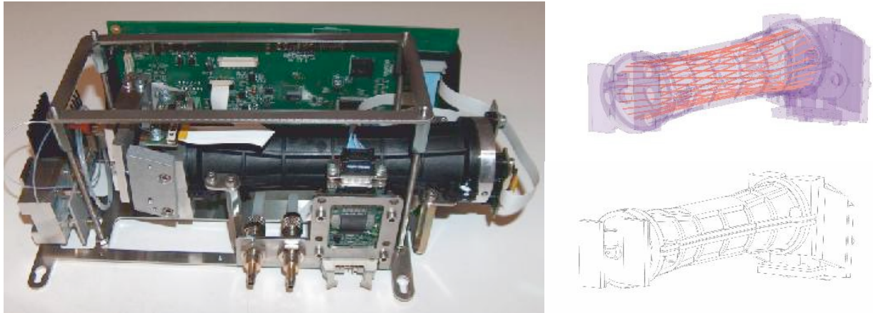
Figure 2. Methane detector, laser diode with Herriot multi-pass cell.
