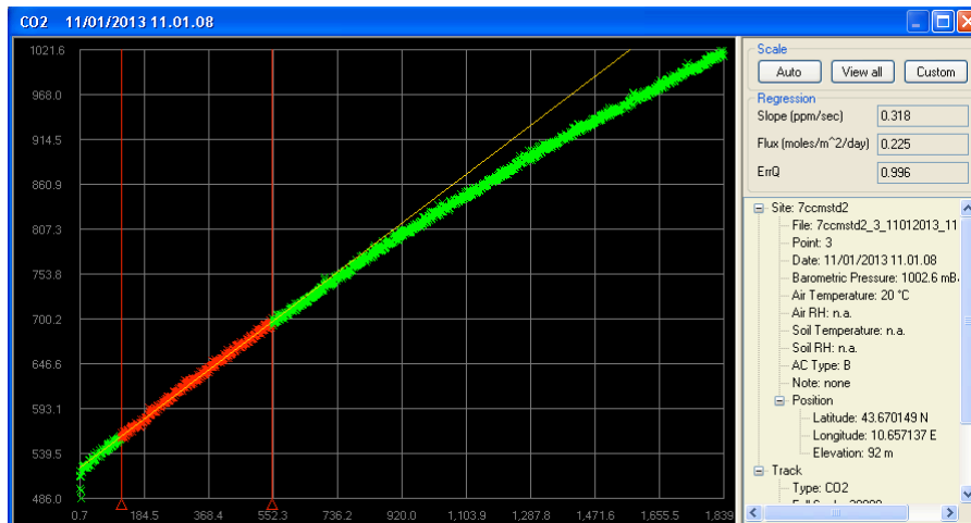
Figure 4. Graphical representation of the increasing concentration value vs time inside accumulation chamber.
