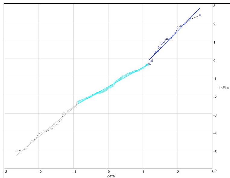
Figure 6. Cumulative probability plots of \text{CH}_4 flux.
