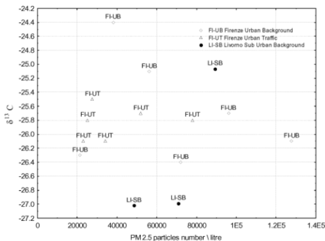
Figure 2- \delta^{13}C value versus total PM2.5 particles number
