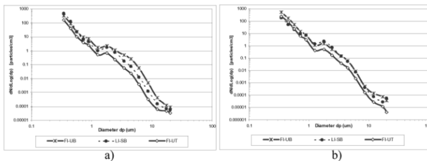
Fig. 1- Observed size distribution for number concentration in a)summer, b) autumn
